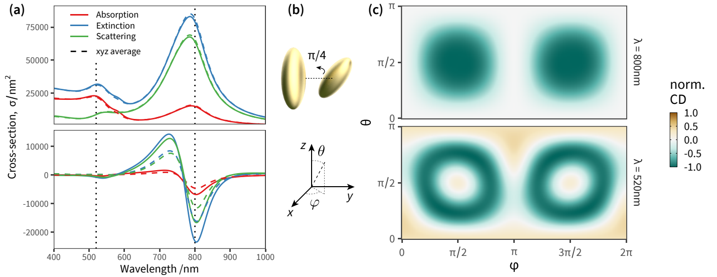
Figure 2 Angular response of a “fingers crossed” dimer of gold spheroids immersed in water (refractive index 1.33). (a) Orientation-averaged far-field extinction (blue), absorption (red), and scattering (green) cross-sections. Lower panel: Orientation averaged circular dichroism spectra. The solid lines correspond to analytical orientation-averaging (exact), while the dashed lines are for the numerical approximation using x, y, z incidence directions only. (b) Schematic representation of the dimer of gold nanorods. Each particle is modelled as a prolate spheroid with semi-axes a = b = 30 nm and c = 80 nm. The first particle is at (0, -100, 0) with major axis along z , while the second particle is at (0, +100, 0) , and tilted from the z axis by a polar angle \theta = \pi/4 . (c) Angular map of the extinction CD at \lambda = 800 nm (upper panel) and \lambda = 520 nm (lower panel). The values are normalised to unity in both panels to facilitate comparison of the patterns. See ESI Fig. S2 † for maps at other wavelengths.
