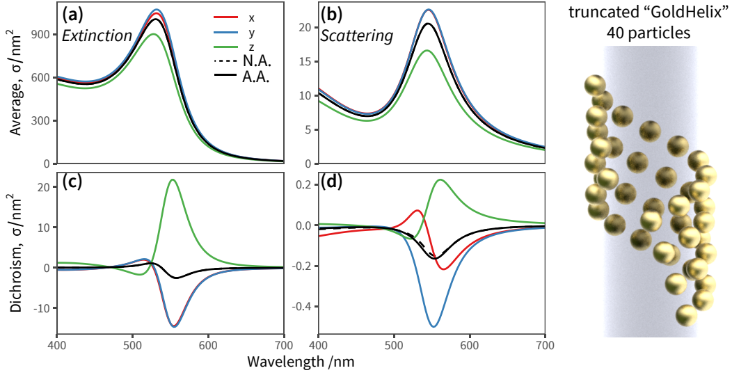
Fig. S3: Angular response of a GoldHelix cluster 2 with N = 40 particles (4 × 10 ribbon). Upper panels: Extinction and scattering spectra for three perpendicular incident directions, x-axis (solid red line), y-axis (solid blue line), z-axis (solid green line), the numerical average over the three (N.A., dashed black line), and the analytical orientation-averaged result (A.A., solid black line). Lower panels: the corresponding results for circular dichroism. Note that the numerical and analytical orientation averages are mostly indistinguishable, except for panel (d).
