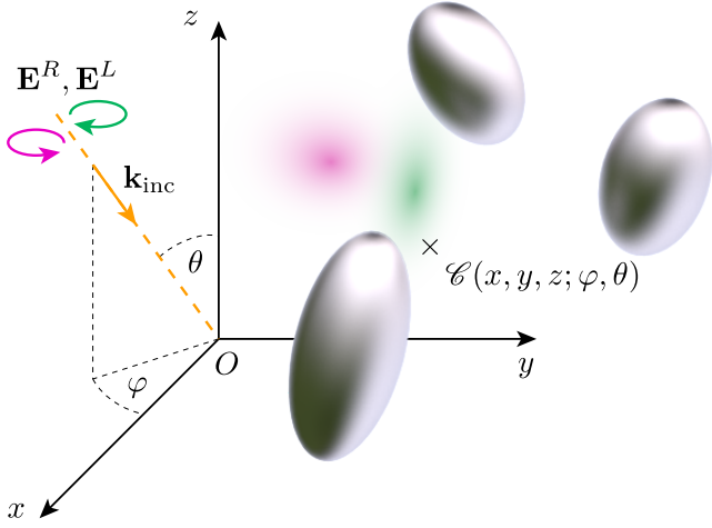
Figure 1 Schematic illustration of the system under study. A cluster of N particles which are placed at arbitrary positions and orientations, is illuminated by incident light in the form of a plane wave with wave vector \mathbf{k}_{\text{inc}} indexed by Euler angles (\theta, \varphi) with respect to a frame attached to the particle cluster. In practice, the particles would be held rigidly in place by a physical support (template); the support’s potential influence on optical properties is assumed to be negligible in this work. We are interested in the variation of the cluster’s optical properties when the incident light changes orientation. We compute far-field cross-sections (total extinction, scattering and absorption) and in particular the differential cross-sections associated with left and right-handed circularly-polarised light (circular dichroism). Another quantity of interest is the near-field local degree of optical chirality \mathcal{C}(x, y, z) for either left- or right-handed incident light.
