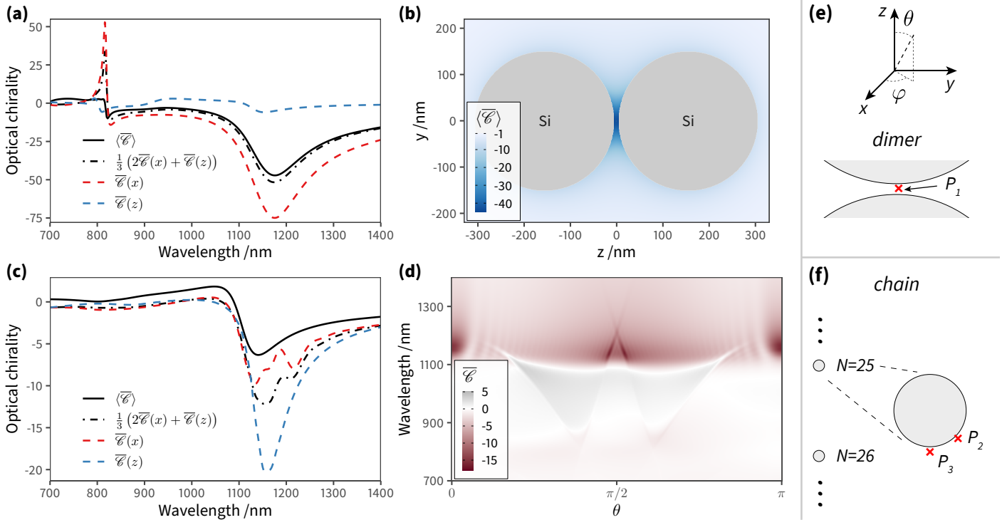
Figure 5 Normalised degree of optical chirality around Si nanospheres of radius r = 150 nm, for a dimer with inter-particle gap = 10 nm and a diffractive chain of 50 Si nanospheres with inter-particle distance d = 1208 nm. The particles are placed in air. (a) Spectrum of \overline{\mathcal{C}} at the point P_1 in the gap between two spheres, 4 nm away of the sphere's surface, as depicted in schematic (e). The structure is illuminated with a right-handed circularly-polarised plane wave incident along the x \equiv y direction (dashed red line), or z direction (dashed blue line). The numerical average over these perpendicular incident directions (N.A., dash-dotted black line) is compared with the analytical orientation-averaged spectrum \langle \overline{\mathcal{C}} \rangle (A.A., solid black line). (b) Map of \langle \overline{\mathcal{C}} \rangle around the dimer, calculated in the y-z plane at the wavelength \lambda = 1175 nm, corresponding to the strongest value of \langle \overline{\mathcal{C}} \rangle in the spectrum. (c) Spectrum of \overline{\mathcal{C}} at the off-axis point P_2 near particle 25 in the 50-particle chain, as depicted in (f). The illumination directions are the same as (a). (d) Dispersion map of \overline{\mathcal{C}} at the point P_3 , varying the incident wavelength and direction \theta .
