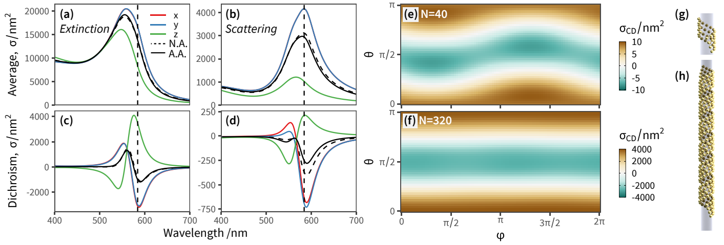
Figure 4 Far-field chiroptical response of a “GoldHelix” cluster described in Ref. [ 58] consisting of a ribbon of 5 nm-radius Au nanospheres wrapped in a helix and immersed in water. The list of particle positions we used is available in ESI † . (a, b) Extinction and scattering spectra for three perpendicular incident directions, x -axis (solid red line), y -axis (solid blue line), z -axis (solid green line), the average over the three (dashed black line), and the analytical orientation averaged result (solid black line). (c, d) The corresponding results for circular dichroism. (e, f) Angular map of circular dichroism (for extinction) for a GoldHelix with number of particles N = 40 (e) and N = 320 (f). (g, h) Schematic illustration of the GoldHelix geometry with N = 40 and N = 320 , respectively. Note that cross-sections are normalised by the number of particles in each cluster, to facilitate comparisons. The simulations considered a maximum multipole order l_{\max} = 4 .
