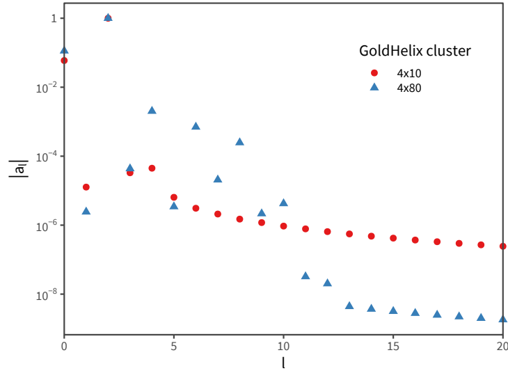
Fig. S4: Spherical harmonic analysis of the circular dichroism angular patterns shown in Fig. 4 (e,f). We use the function sphharm from the Matlab library chebfun 3,4 to compute the decomposition of the angular map into spherical harmonics. For each harmonic degree l we collapse the corresponding 2l + 1 orders as |a_l| = \sum_{m=-l}^l |a_{lm}|^2 ; the result summarises the total weight of degree l in the pattern (higher degrees correspond to higher angular frequencies). For ease of comparison the scale is logarithmic, and we normalise the results such as \max a_l = 1 . The two cases considered correspond to the full GoldHelix cluster (blue triangles, 320 particles), and the truncated structure (red circles, 80 particles).
