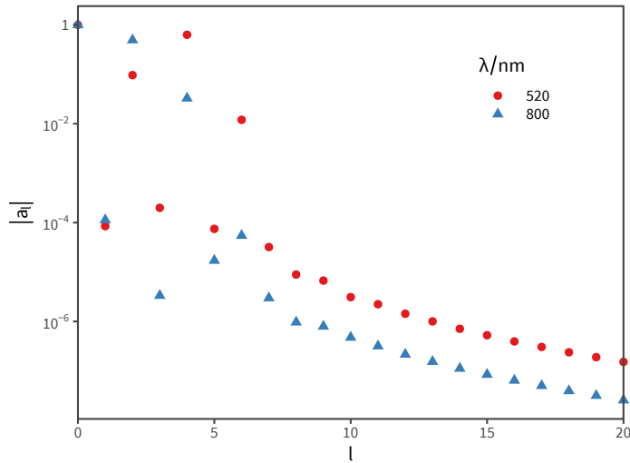
Figure 3 Spherical harmonic analysis of the circular dichroism angular patterns shown in Fig. 2(c). We use the function sphharm from the Matlab library Chebfun 54,55 to compute the decomposition of the angular map into spherical harmonics. For each harmonic degree l we collapse the corresponding 2l + 1 orders as |a_l| = \sum_{m=-l}^l |a_{lm}|^2 ; the result summarises the total weight of degree l in the pattern (higher degrees correspond to higher angular frequencies). For ease of comparison the scale is logarithmic, and we normalise the results such as |a_0| = 1 . The two cases considered correspond to \lambda = 520 nm (red dots) and \lambda = 800 nm (blue triangles).
