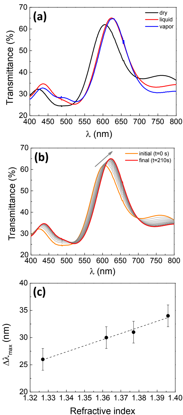
Figure 6. (a) UV-Visible spectra of 4x(SC/TF)/Au/TSV measured dry, in an atmosphere saturated with butanol vapour and after immersion in liquid butanol. (b) UV-visible spectra of the same device as a function of time in contact with liquid butanol. The orange curve corresponds to the initial state (dry, t=0 s) and the red one to the final state (full of solvent, t=210 s). (c) Linear calibration curve for the variation of the Tamm plasmon peak position of the protected device as a function of refractive index for different vapours (alcohols) filling the pores.
