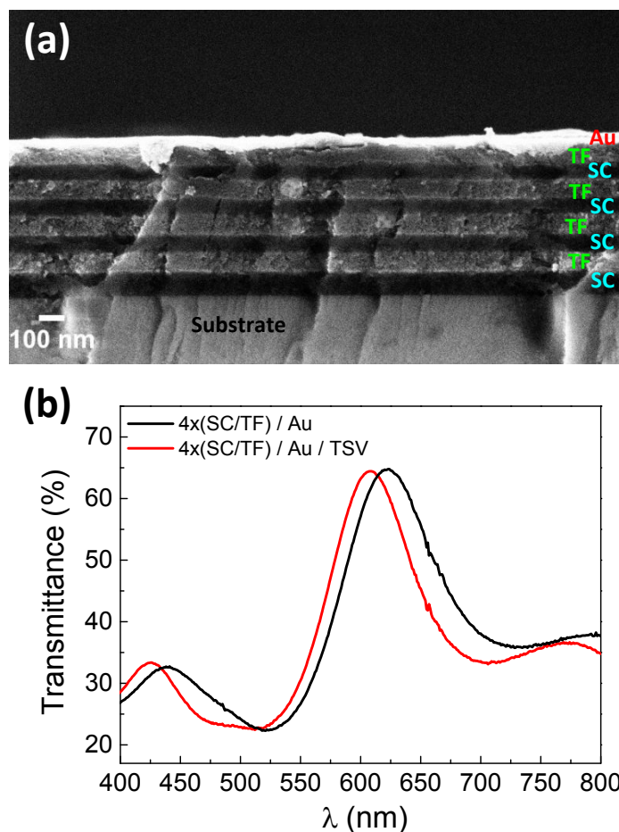
Figure 3. (a) Cross sectional SEM micrograph of 4x(SC/TF)/Au device. (b) Transmittance spectra of 4x(SC/TF)/Au and 4x(SC/TF)/Au/TSV devices, measured at 0% relative humidity.
