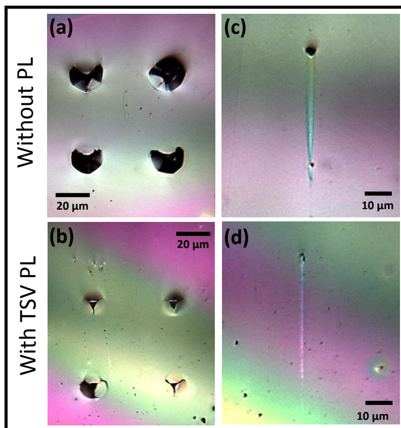
Figure 5. Optical microscopy photographs of the surface of Tamm plasmon devices with and without PL. Array of 4 indentations up to 1000 nm depth in 4x(SC/TB)/Au ( a ) and 4x(SC/TB)/Au/TSV ( b ); scratches in the same Tamm plasmon devices, without ( c ) and with ( d ) TSV PL.
