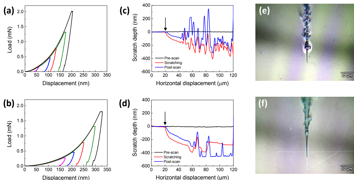
Figure 2. Selected load vs displacement measurements (ISO method, maximum load of 2 mN) for ZF (a) and TSV (b). Examples of scratch measurements (c,d) and optical images (e,f) of the performed scratches for ZF (c, e) and for TSV (d,f), up to a maximum load of 5 mN. The arrows indicate the beginning of the scratching.
