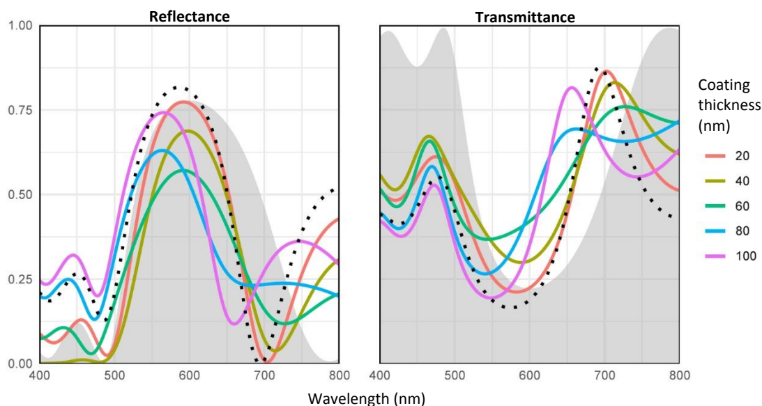
Figure 1. Variation of the reflectance (left) and the transmittance (right) spectra of a Tamm plasmon device (dotted line) with the incorporation of a superficial PL of different thicknesses from 20 to 100 nm. The grey shadows represent the corresponding DBR spectra ( i.e. the device without the Au layer). The dotted black line corresponds to the bare TPP structure (no PL layer).
