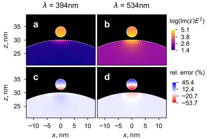
Figure 2 Near-field intensity maps at resonance for the absorption by a Au core and a Ag satellite for two wavelengths: \lambda = 394 \text{ nm} (a) and \lambda = 534 \text{ nm} (b). The calculations were performed with TERMS, using a maximum multipolar order of 40. The bottom panels (c,d) show the corresponding relative error resulting from using a dipole approximation to describe the satellite's optical response. This was obtained by simulating the cluster with TERMS and setting the T -matrix coefficients describing the satellite particle, but not the core particle, to zero, for all but the electric dipole coefficient. The error is obtained by subtracting the converged solution displayed above. Note the linear scale in panels (c-d).
