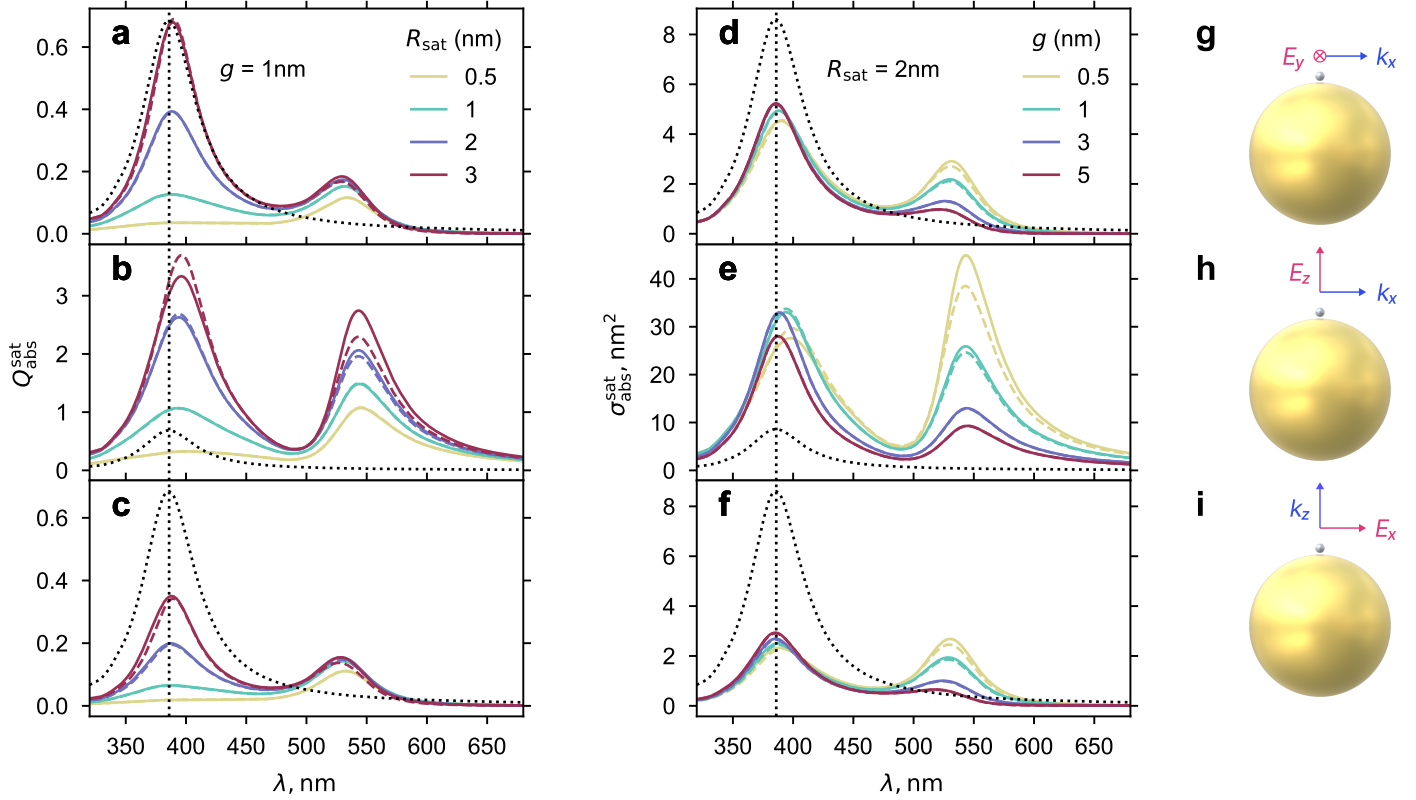
Figure 3 Effect of the satellite radius R_{\text{sat}} for a fixed gap of g = 1 nm (a–c) and the gap between the satellite and the core sphere for a fixed radius of R_{\text{sat}} = 2 nm (d–f) on partial absorption spectra, for a Au–Ag core–satellite structure. Solid lines correspond to rigorous spectra calculated with TERMS, and dashed lines using GCDM. In panels (a–c), the partial absorption cross-section \sigma_{\text{abs}}^{\text{sat}} is normalised by the geometrical cross-section \sigma_{\text{geo}} = \pi R_{\text{sat}}^2 . The unit-less partial absorption efficiency Q_{\text{abs}}^{\text{sat}} := \sigma_{\text{abs}}^{\text{sat}} / \sigma_{\text{geo}} is used to ease the comparison between different satellite radii, as the absorption augments rapidly with the particle radius. The dotted line shows the position of the main peak of a single silver satellite without a core particle, for reference. The absorption spectrum of an isolated Ag satellite in water is also show for comparison (dotted curve, identical across all panels). Rows of the plots (a–f) correspond to different cases of the incidence on the particle illustrated in schemes (g–i).
