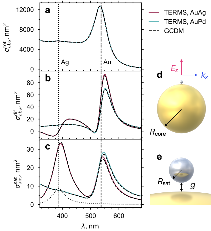
Figure 1 Absorption spectra for a single Ag or Pd satellite of radius R_{\text{sat}} = 2 \text{ nm} , next to a spherical Au core particle of radius R_{\text{core}} = 30 \text{ nm} , separated by a gap g = 1 \text{ nm} . The particles are immersed in water. (a) Total absorption cross-section for the whole structure. (b) Differential absorption cross-section (Eq. 4). (c) Partial satellite absorption cross-section. GCDM calculations (dashed lines) are compared to the rigorous T -matrix solution of Maxwell's equations using the TERMS program 40 (solid lines). The vertical dotted lines indicate the spectral position of the plasmon resonance of an isolated Au or Ag sphere in water, for reference. The absorption spectrum of an isolated Ag satellite in water is also shown for comparison (dotted curve). (d) Geometry of the particle with a single Ag satellite on the Au core and the incident light propagating along the x axis with z -polarised electric field. (e) Close-up view of the satellite near the core particle.
