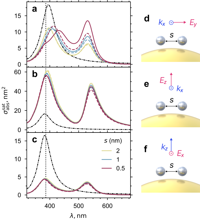
Figure 4 Partial absorption spectra for two satellites with varying separation s . Solid lines correspond to spectra calculated with TERMS and dashed lines with GCDM. The dotted vertical line shows the position of the main peak of a single silver satellite without a core particle. The dash-dotted spectrum shown for reference corresponds to the two silver satellites with no core Au particle present. Panels (a–c) correspond to different orientations of the incident light, illustrated in the corresponding schemes (d–f).
