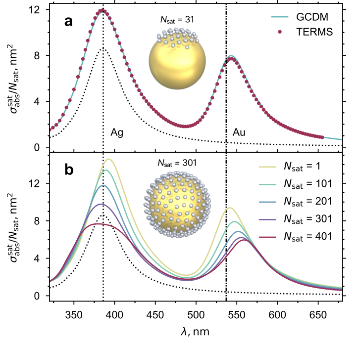
Figure 5 Influence of the number of satellites N_{\text{sat}} . (a) Validation of the GCDM model against TERMS for the partially covered core particle with a dense coverage of 31 satellites equivalent to a full coverage of standard core-satellite structure with 301 satellites (structure shown in inset). (b) GCDM calculations for a fully-covered spherical core, with varying numbers of satellites. Spectra were calculated using numerical orientation averaging 48 for the incident light. Correspondences of the number of satellites and their minimal inter-satellite separation are as follows: N_{\text{sat}} = 101, s \approx 6.2 nm; N_{\text{sat}} = 201, s \approx 3.2 nm; N_{\text{sat}} = 301, s \approx 1.9 nm; N_{\text{sat}} = 401, s \approx 1.1 nm.
